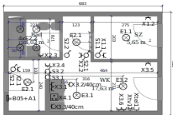
House wiring layout plan
