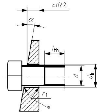
Bolt clamp test fixture
